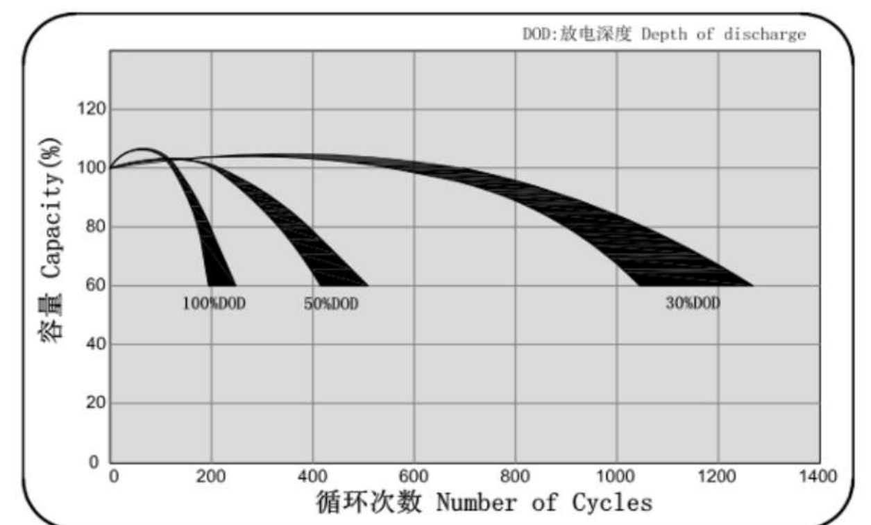
Cycle Life Relation to Depth of Discharge
