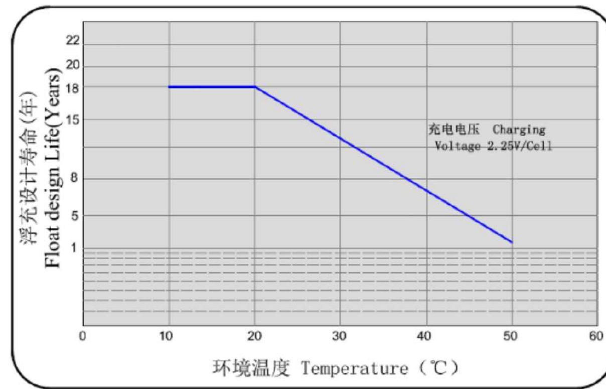
Effect of Temperature on Float Life
