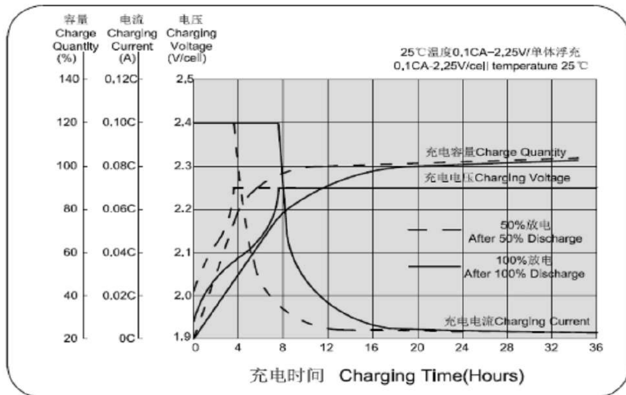
Float Charging Characteristics
